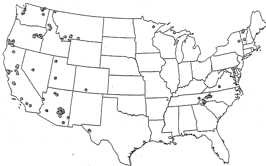
Figure 2. Occurrences of asbestos in the contiguous United States. Major asbestos-bearing deposits occur in the mountain belts in the Eastern and Western United States. Data from ISGS Digital Data Series DDS-52 (E.J. McFaul and others, 2000, U.S. Geological Survey Mineral Databases—MRDS and MAS/MILS).
