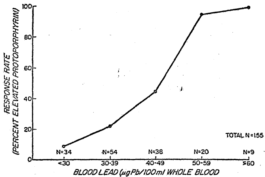
FIGURE 2. Dose-response relationship for the effects of internal doses of lead as Pb-B on erythrocyte protoporphyrin.
