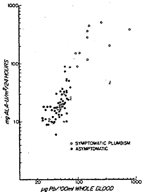
FIGURE 1. Dose-effect relationship between an indicator of internal dose (Pb-B) and an indicator of effect (urinary excretion of ALA, ALA-D).
