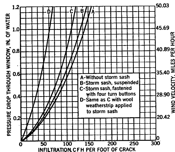
FIG. 4. INFILTRATION THROUGH SASH PERIMETER OF WINDOW WITH AND WITHOUT STORM SASH— \frac{5}{64} -IN. CRACK AND \frac{1}{32} -IN. CLEARANCE
