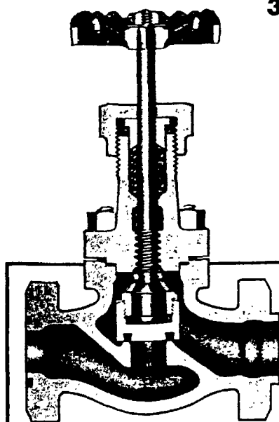
Cross-section bolted bonnet Globe, with flanged ends and special lead-faced disc. Sizes 1/2 to 4-inch.
