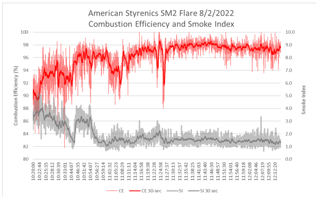
Figure 2: Combustion Efficiency and Smoke Index for the SM2 flare on 8/2/2022.
