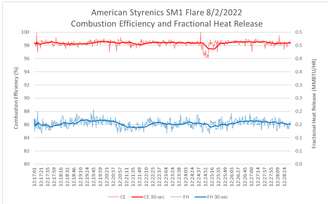
Figure 3: Combustion Efficiency and Fractional Heat Release for the SM1 flare on 8/2/2022.
