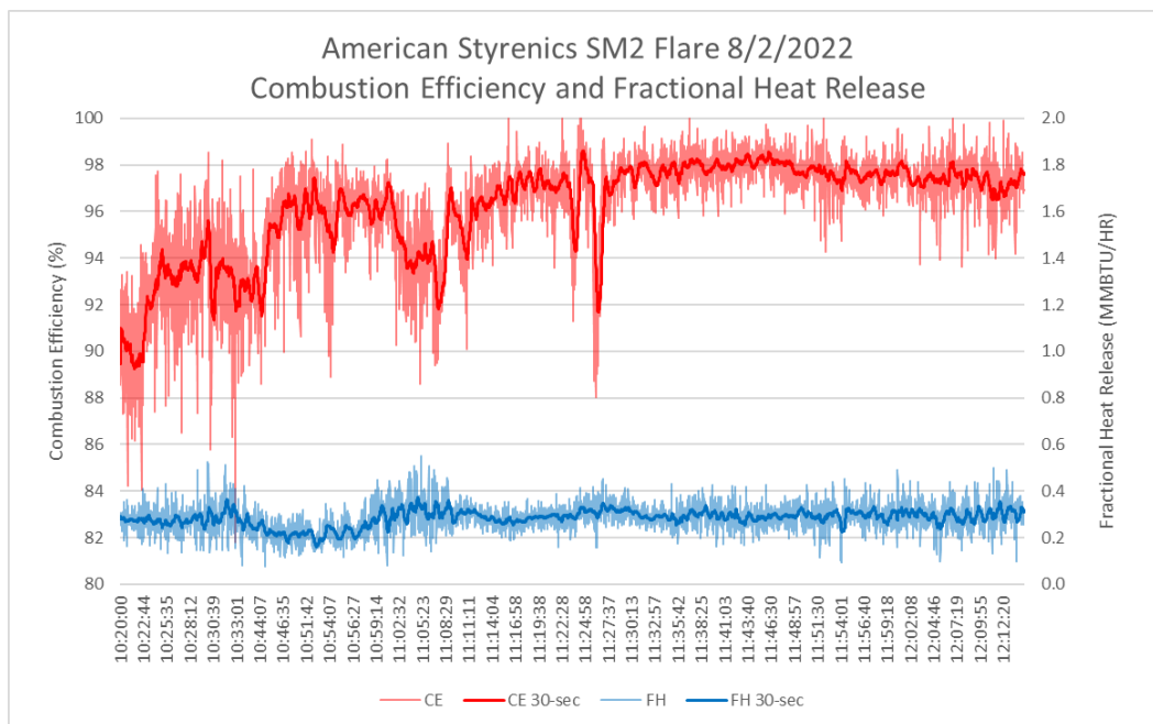
Figure 1: Combustion Efficiency and Fractional Heat Release for the SM2 flare on 8/2/2022.
