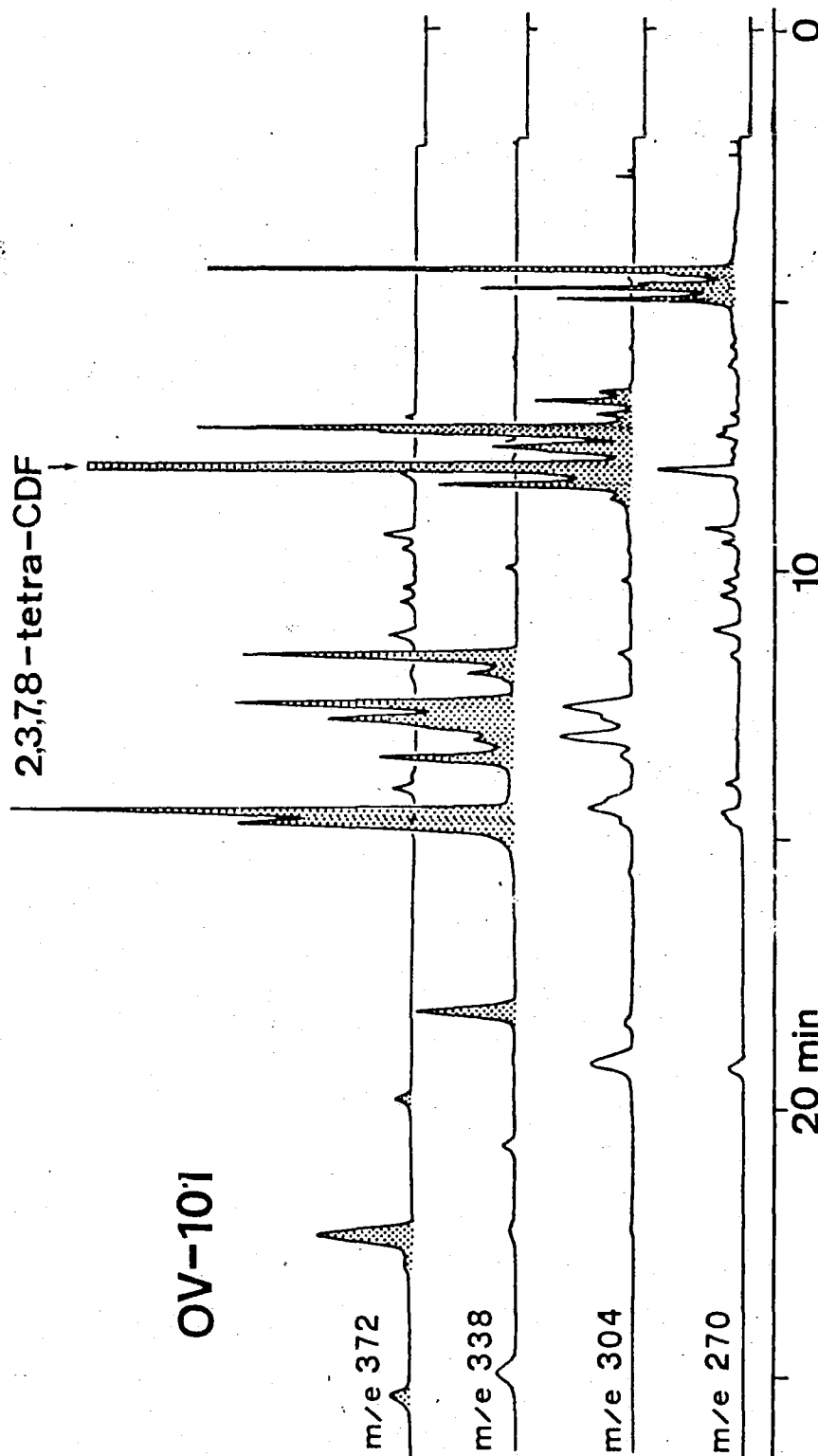
Figure 1 : Mass fragmentograms (OV-101 glass capillary columns at 197°C) of Yusho oil showing elution of PCDFs (m/e 270 = tri-, m/e 304 = tetra-, m/e 338 = penta- and m/e 372 = hexa-CDF).
