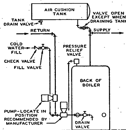
FIG. 16. A CLOSED EXPANSION TANK
