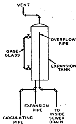
FIG. 15. AN OPEN EXPANSION TANK
