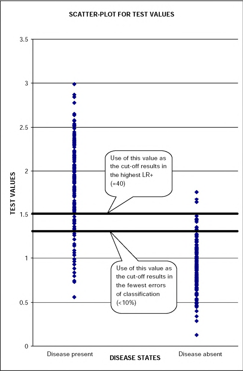
Figure 4. Scatter-plot for test results on 150 people with a certain disease and 150 without the disease
