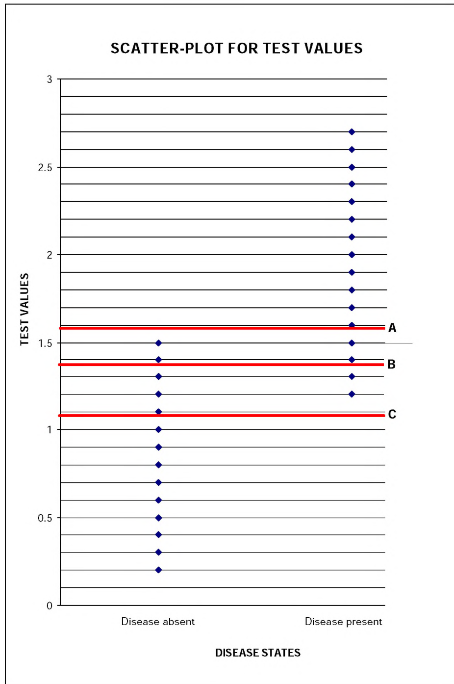
Figure 1: Scatter-plot of hypothetical test results (14 non-diseased, 16 diseased individuals)
