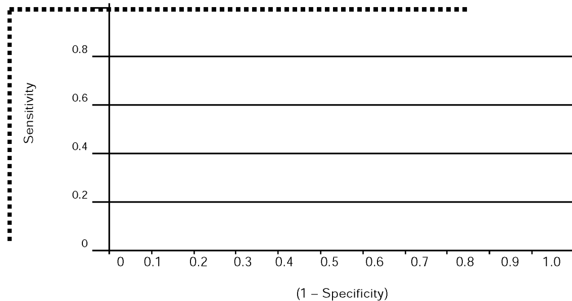
Figure 2: ROC curve for a perfectly discriminating test
