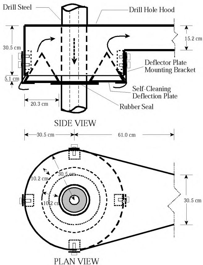
Figure 1. Inlet hood design tested in laboratory.
