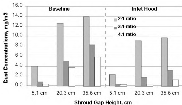
Figure 2. Dust escaping the laboratory drill shroud.
