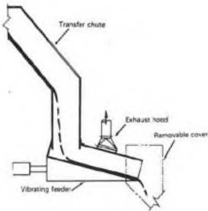
Vibrating Feeder
