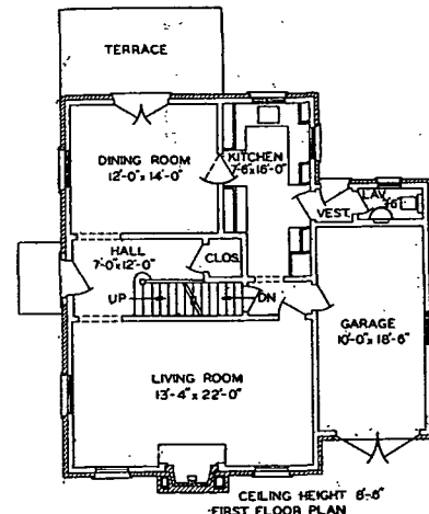
FIG. 2. FLOOR PLANS OF RESIDENCE
