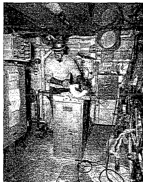
FIGURE 3. Sawing pipe sections.
