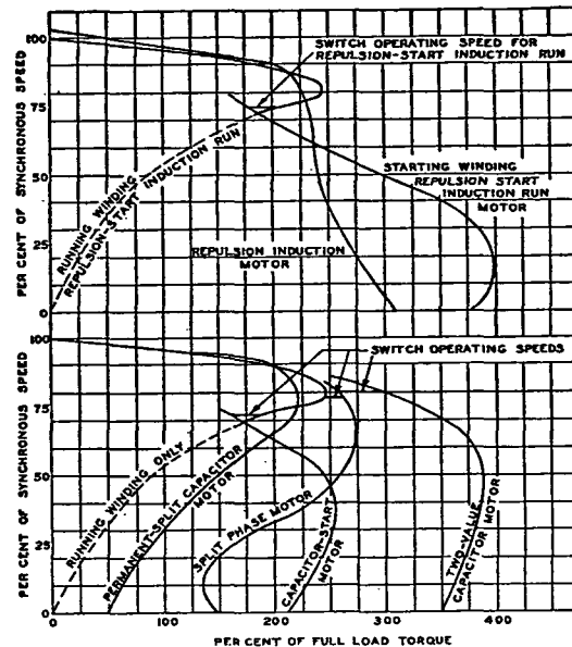
FIG. 4. SPEED-TORQUE CHARACTERISTICS OF SINGLE PHASE MOTORS
