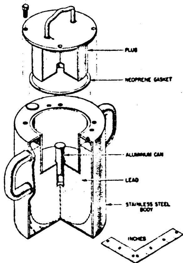
FIGURE 7 RETURNABLE CONTAINER FOR UNSEPARATED ISOTOPES (Reactor Unit) FOR LARGER QUANTITIES
