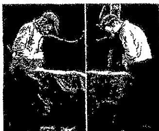
Figure 2. Left: Operator in monument shed using pneumatic barker. Neither dust control nor respirator has been provided. Right: The same operation with goggles and dust-control hood in use.
