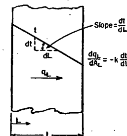
FIG. 2. THERMAL CONDUCTION IN A FLAT SLAB
