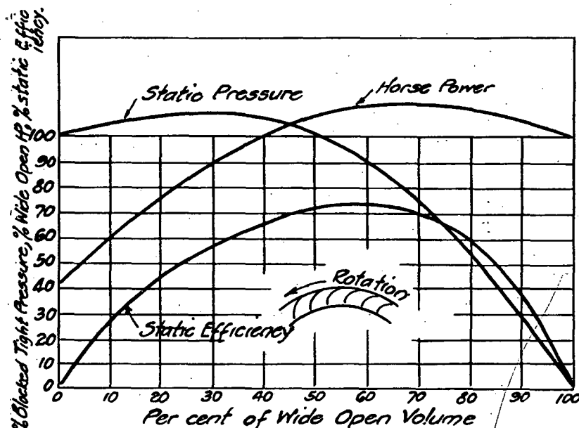
FIG. 7. OPERATING CHARACTERISTICS OF A FAN WITH FULL BACKWARD CURVED BLADES
