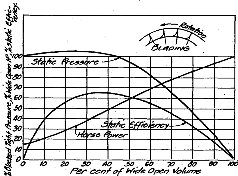
FIG. 6. OPERATING CHARACTERISTICS OF A FAN WITH RADIAL TIE BLADES
