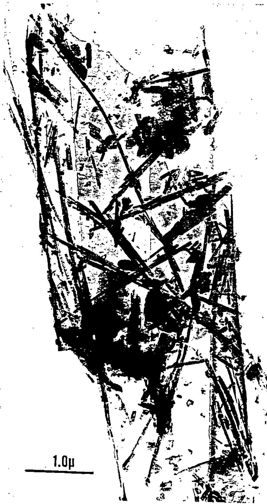
Fig 2.—Clay particle with adsorbed chrysotile fibrils, in air sample about construction site ( \times 28,000 ).
