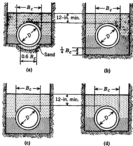
Fig. A2. Bedding Conditions Illustrated
