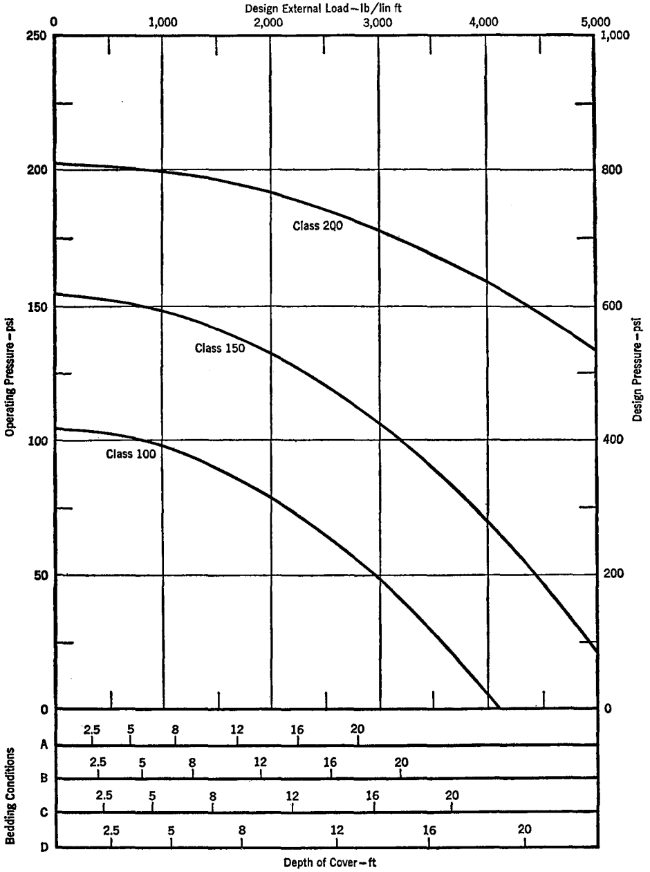
Fig. 7. Selection Curves for 4-in. Asbestos-Cement Pipe
