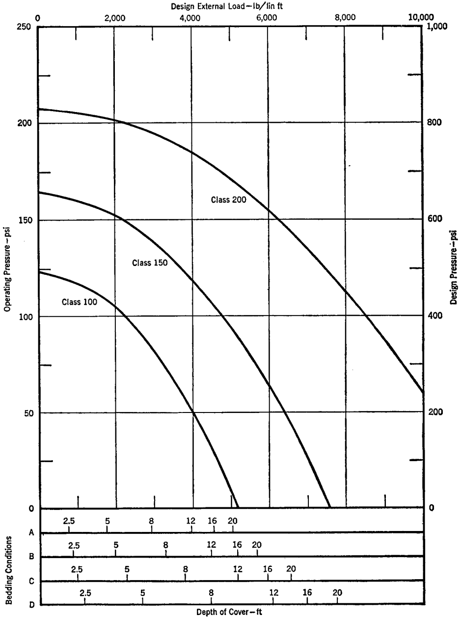
Fig. 11. Selection Curves for 12-in. Asbestos-Cement Pipe
