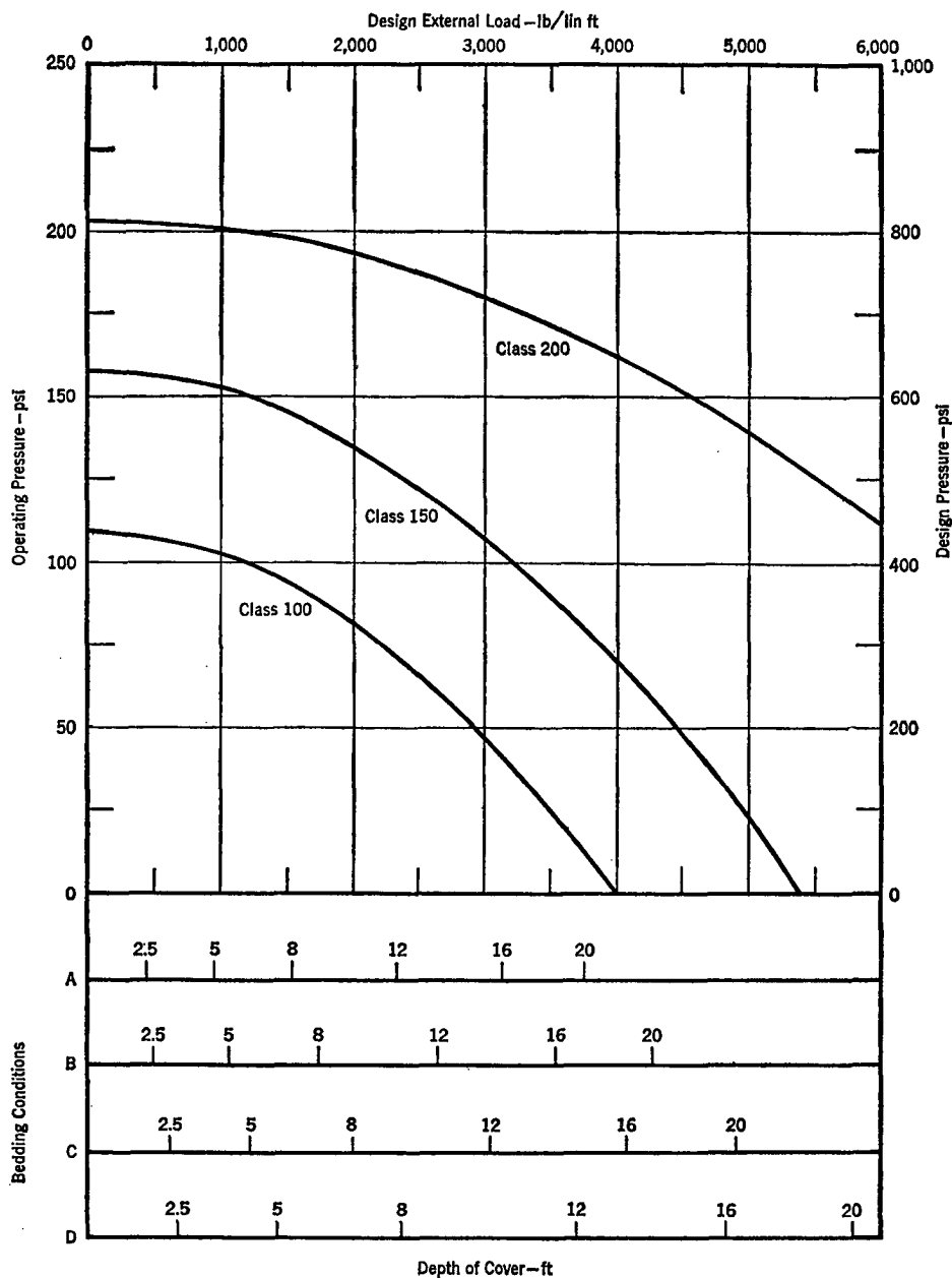
Fig. 8. Selection Curves for 6-in. Asbestos-Cement Pipe
