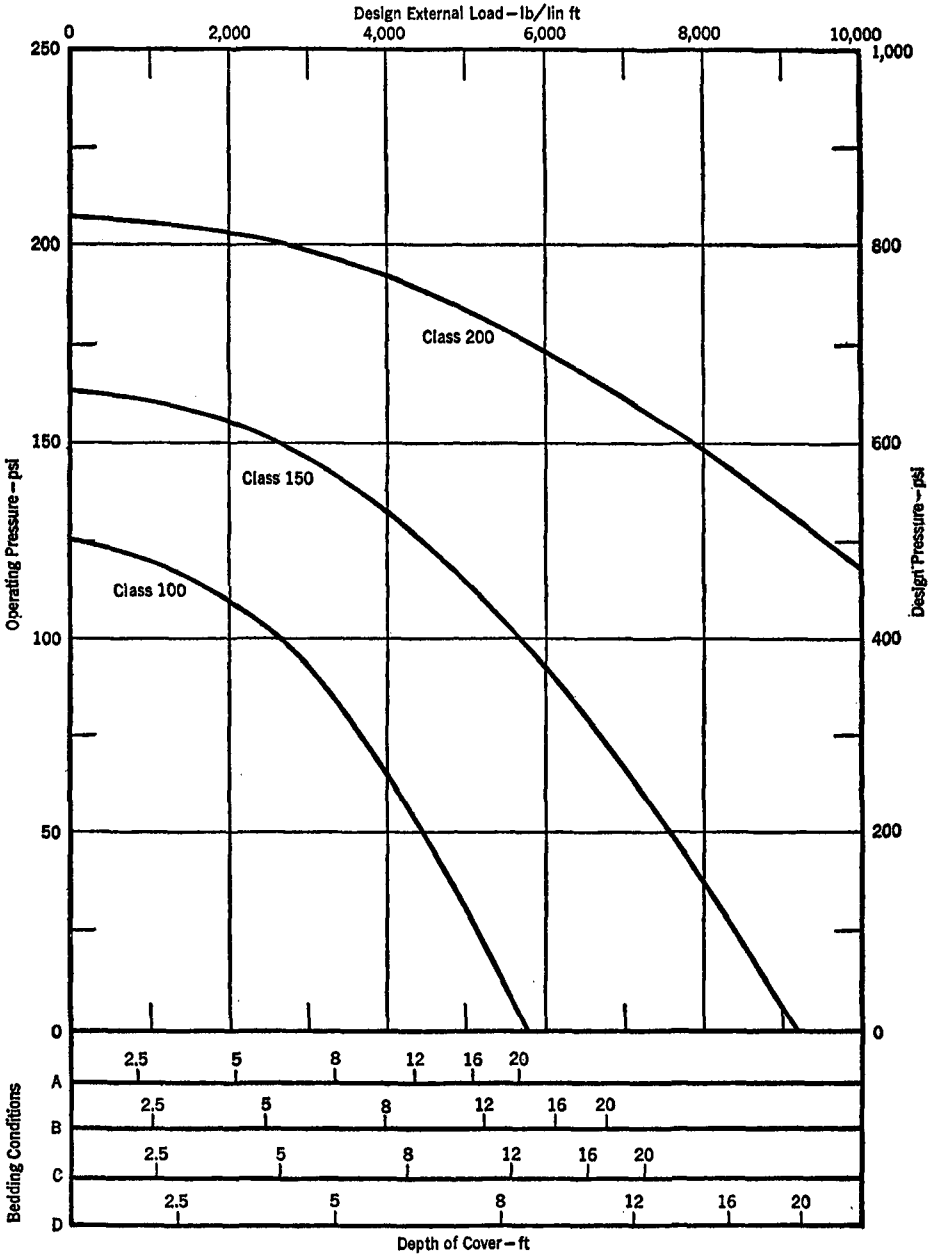
Fig. 13. Selection Curves for 16-in. Asbestos-Cement Pipe
