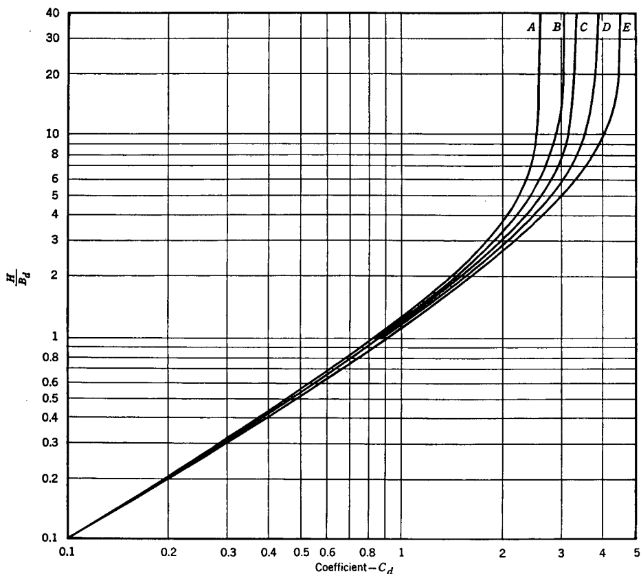
Fig. 4. Graph for Determining C_d Coefficients
