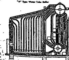
2-Drum Water Tube Boiler
