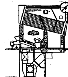
Horizontal Cross or Long Drum Water Tube Boiler
