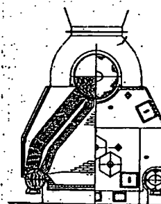
'A' Type Water Tube Boiler for Marine Use
