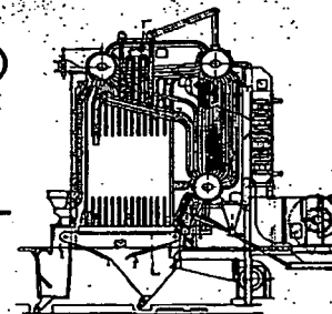
2-Drum 'Y' Type Water Tube Boiler
