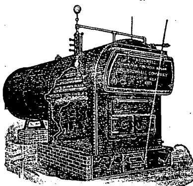
Brownell Return Flue Portable—Direct Draft Type—Bulletin B-6A
