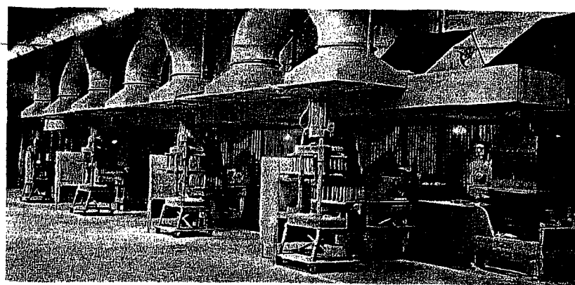
Figure 7. In this foundry, local exhaust hoods are installed over each station having a shell-molding machine and glue press. Adequate make-up air is supplied from ventilating duct situated between molding machines and presses. (Courtesy American Foundrymen's Society)
