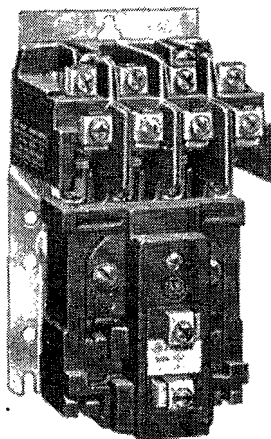
BULLETIN 760 Type BR 4-pole control relay with convertible contacts
