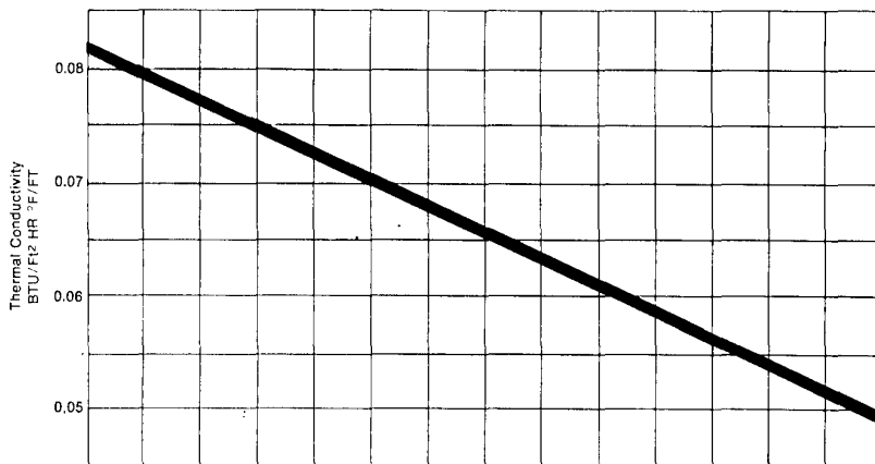
Thermal Conductivity of Liquid Therminol® VP-1
