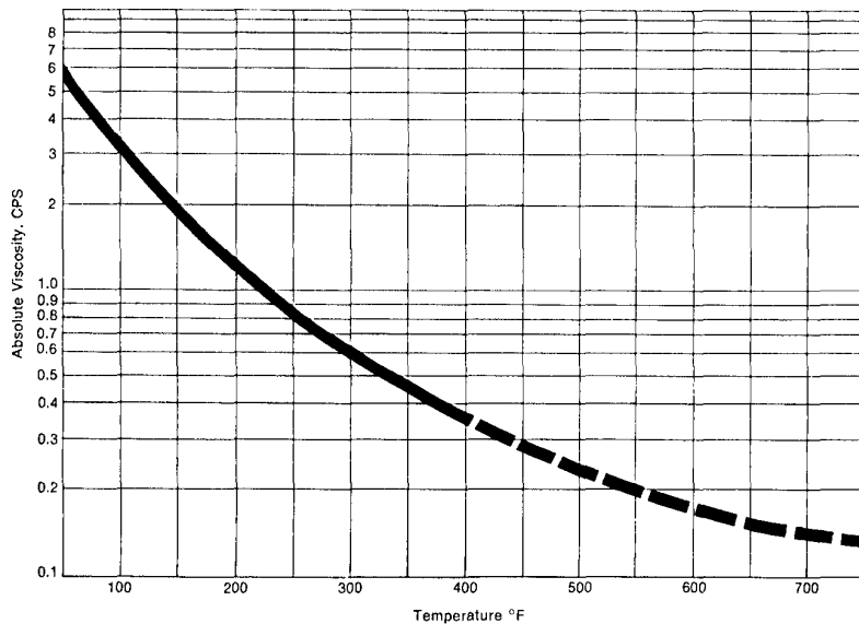
Viscosity of Liquid Therminol® VP-1
