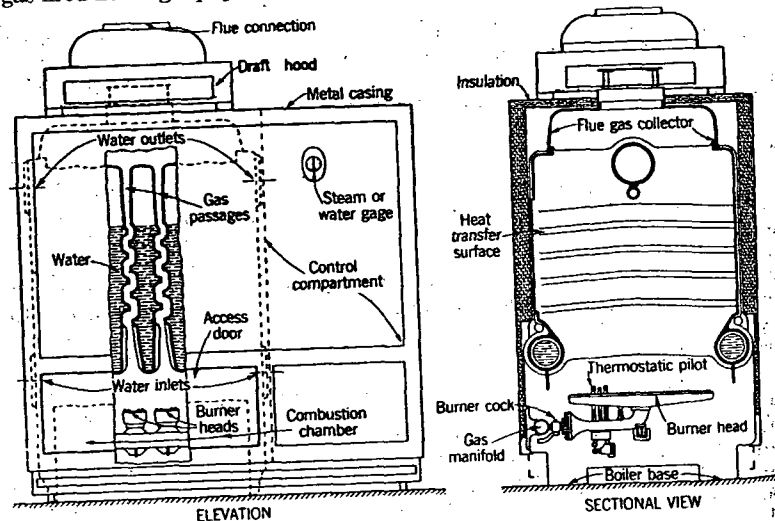
FIG. 19. GAS-FIRED BOILER
