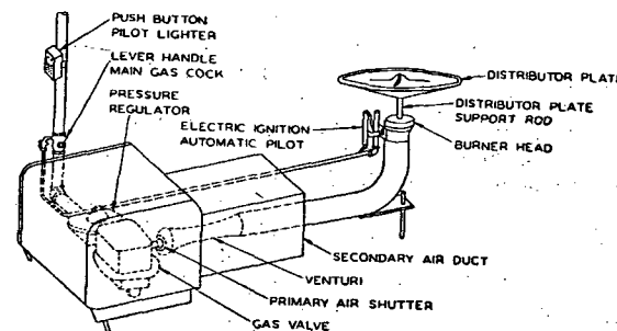
FIG. 20. TYPICAL SINGLE PORT GAS CONVERSION BURNER
