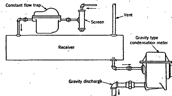
FIG. 6. GRAVITY INSTALLATION FOR CONDENSATE METER USING VENTED RECEIVERS
