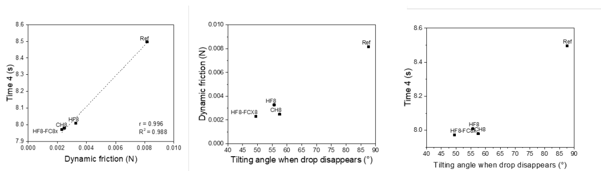
Figure 10. Selection of correlation plots between glide time, dynamic friction and contact angle measurements (here shown as the tilting angle of the base when the water drop disappears). There is a greater difference between no ski wax and ski wax than between ski wax with and without fluorine in all tests.
