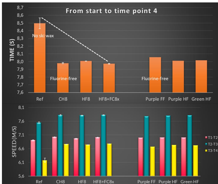
Figure 9. Total glide time and calculated speeds between the different gates in the glide performance testing in the Mid Sweden 365 ski tunnel in Gällö.
