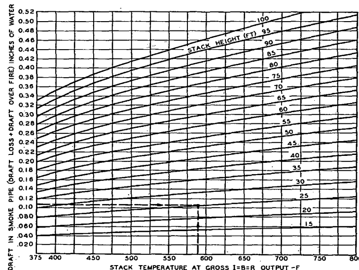
Fig. 8....Stack Height Selection for Automatically Fired Boilers
