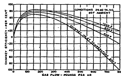
Fig. 7....Effect of Gas Flow on Chimney Efficiency*
