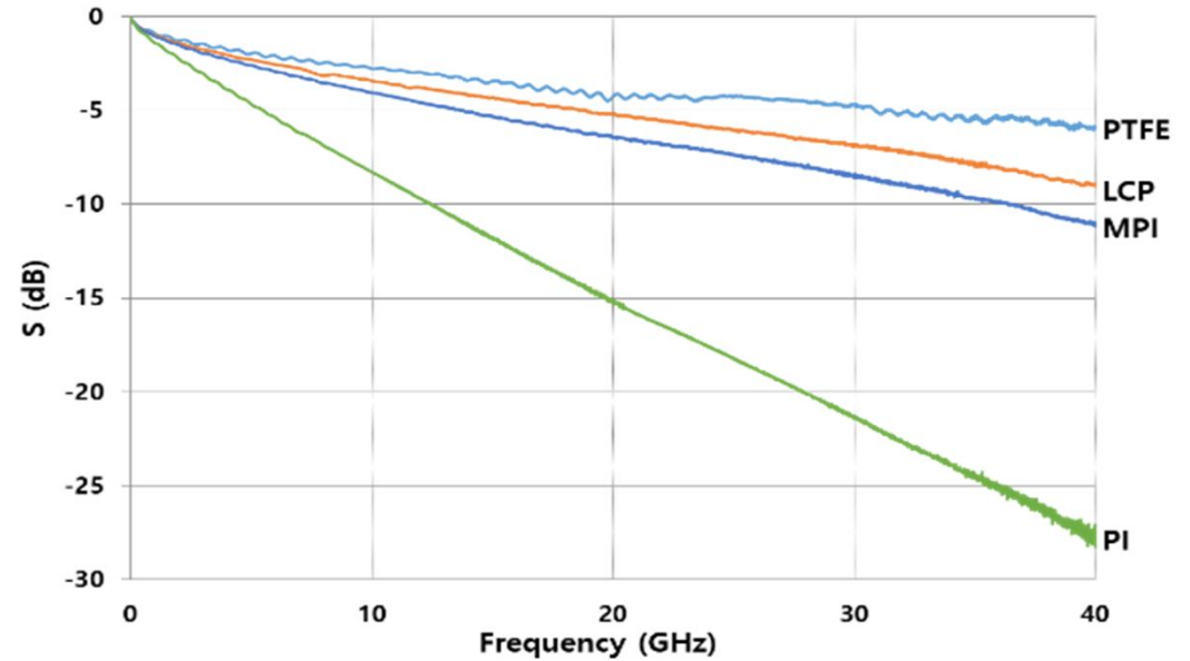
Fig 3. Insertion Loss according to material type
