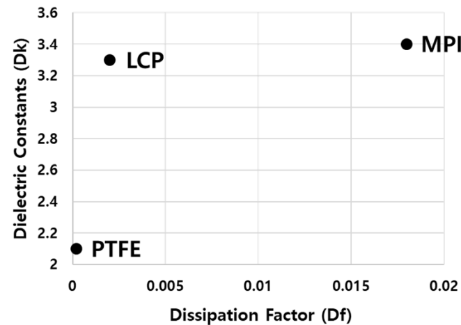
Fig 2. Dielectric constants and Dissipation factor of the resins used for printed circuit boards
