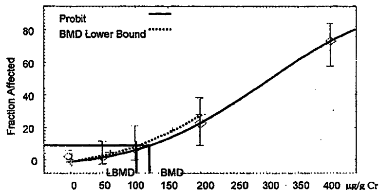
Fig. 1. Probit Model the dose response relationship between UAs and UALB with 0.95 confidence level and the BMD-10 and LBMD-10 are indicated.
