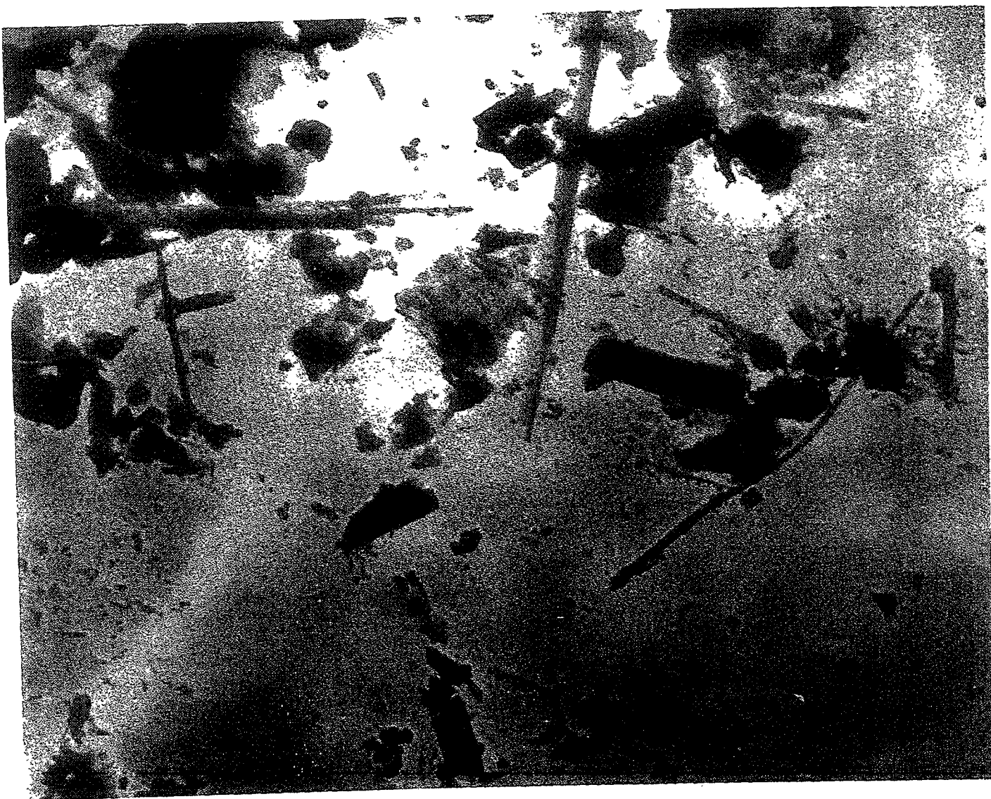
Figure 3. Electron Photomicrograph of Airborne Particulates in Mine and Mill
