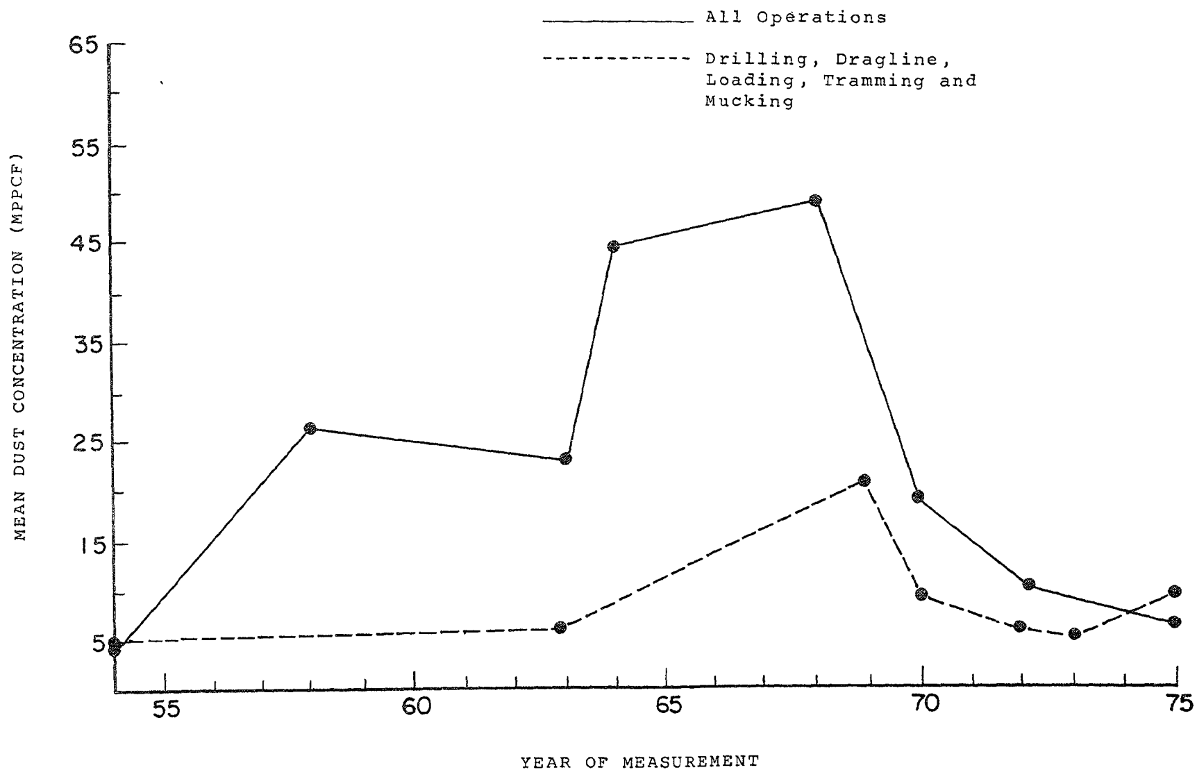
Figure 6. Mean Yearly Impinger Dust Concentrations for Mine Operations
