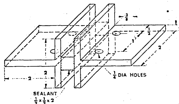
FIG. 4—Assembly for Testing Adhesive Strength to T-Sections.
