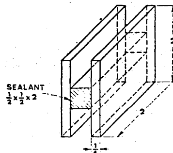
FIG. 3—Assembly for Testing Adhesive Strength to \frac{1}{4} -Inch Plate.
