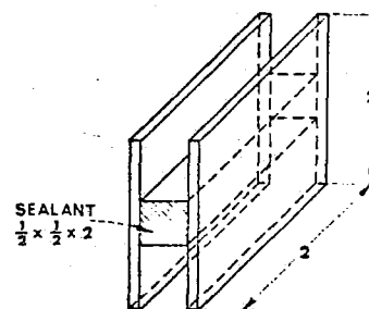
FIG. 5—Assembly for Testing Adhesive Strength to Thin Plates.
