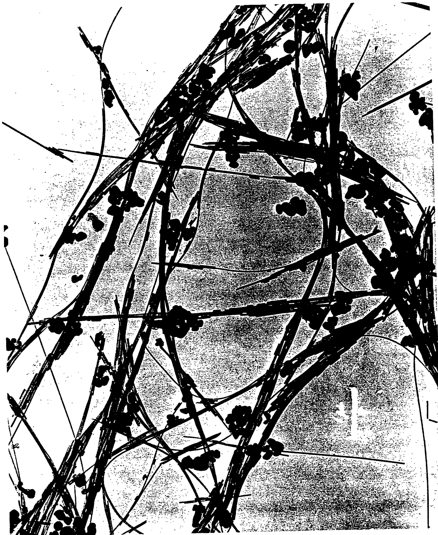
Electron Micrograph of Titanated Asbestos, CALIDRIA Type T-135
