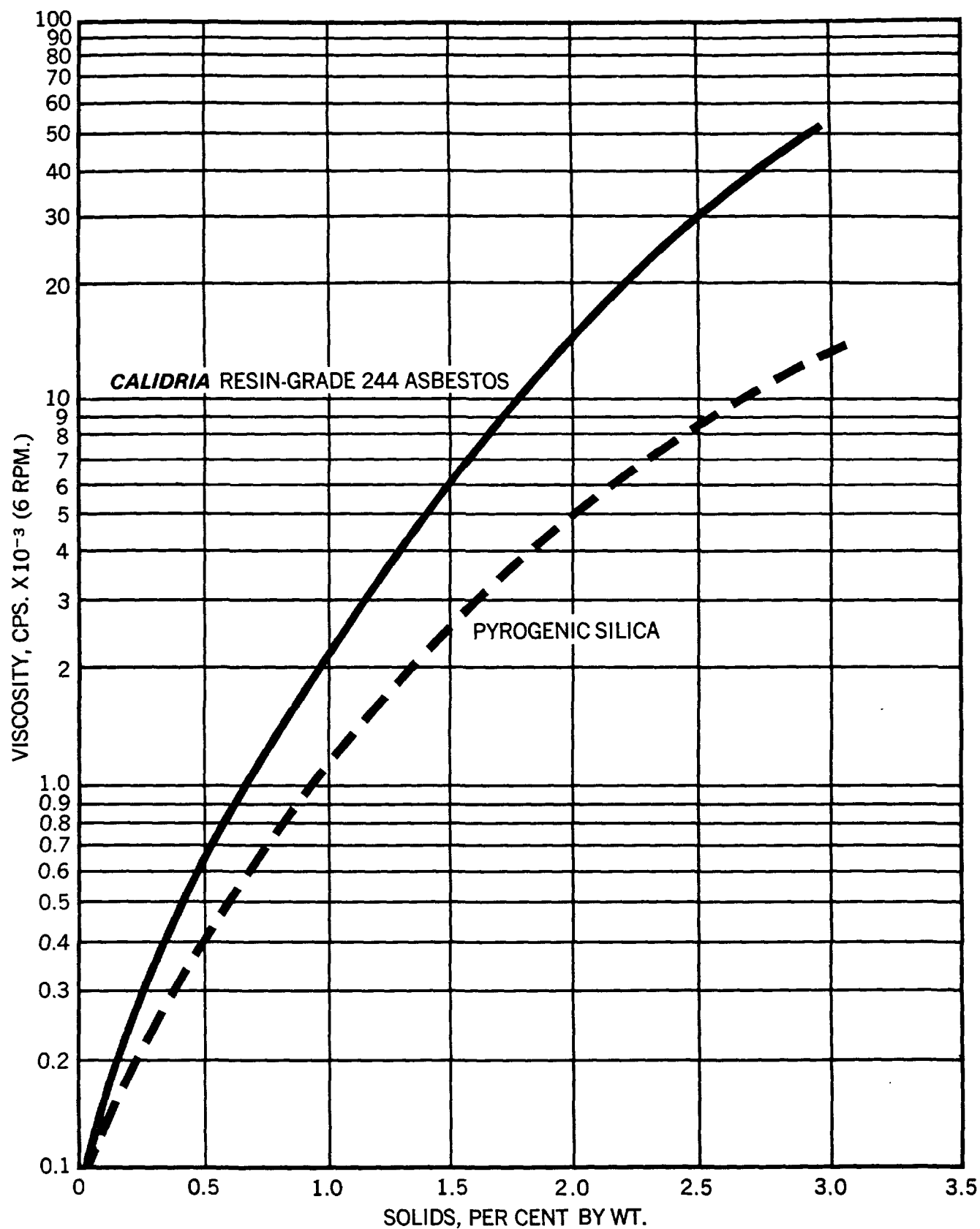
Comparison of Thickening Efficiency of Resin-Grade 244 Asbestos with that of Colloidal Silica in Polyester Resin
