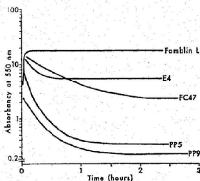
Fig. 1. Emulsion absorbance plotted against ultrasonication time. Emulsions were circulated through a Branson autotuned sonicator cell at 10°C, sample streams were flowed through spectrophotometer cuvettes having appropriate light paths, and the optical density was recorded. The optical density was calculated to account for the length of the cell path.
