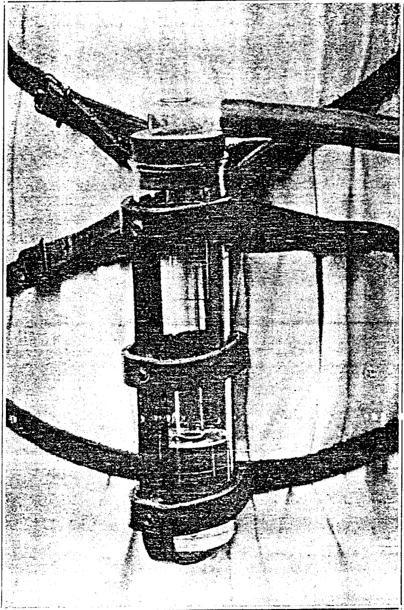
LEATHER HOLSTER WITH IMPINGER IN PLACE
