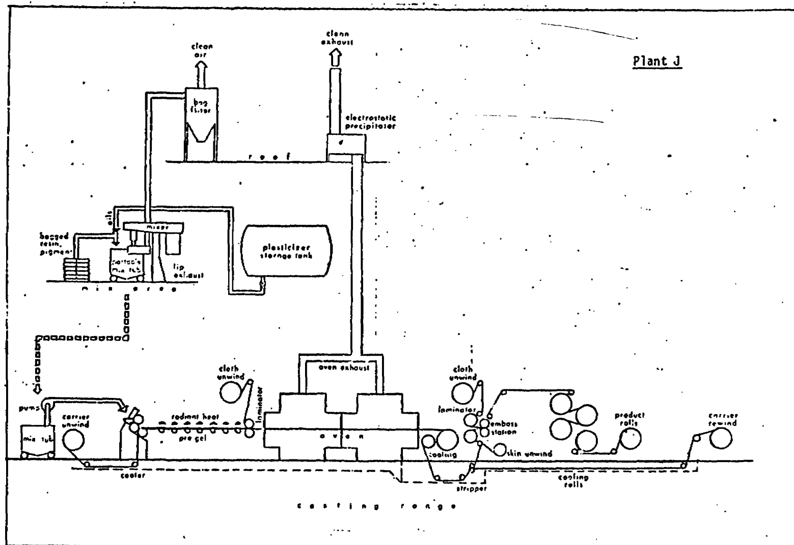
Figure 13. Flow Schematic, Cast Film Production, Plant J
