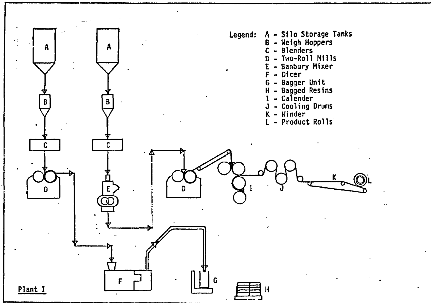
Figure 12. Flow Schematic, Plant I
