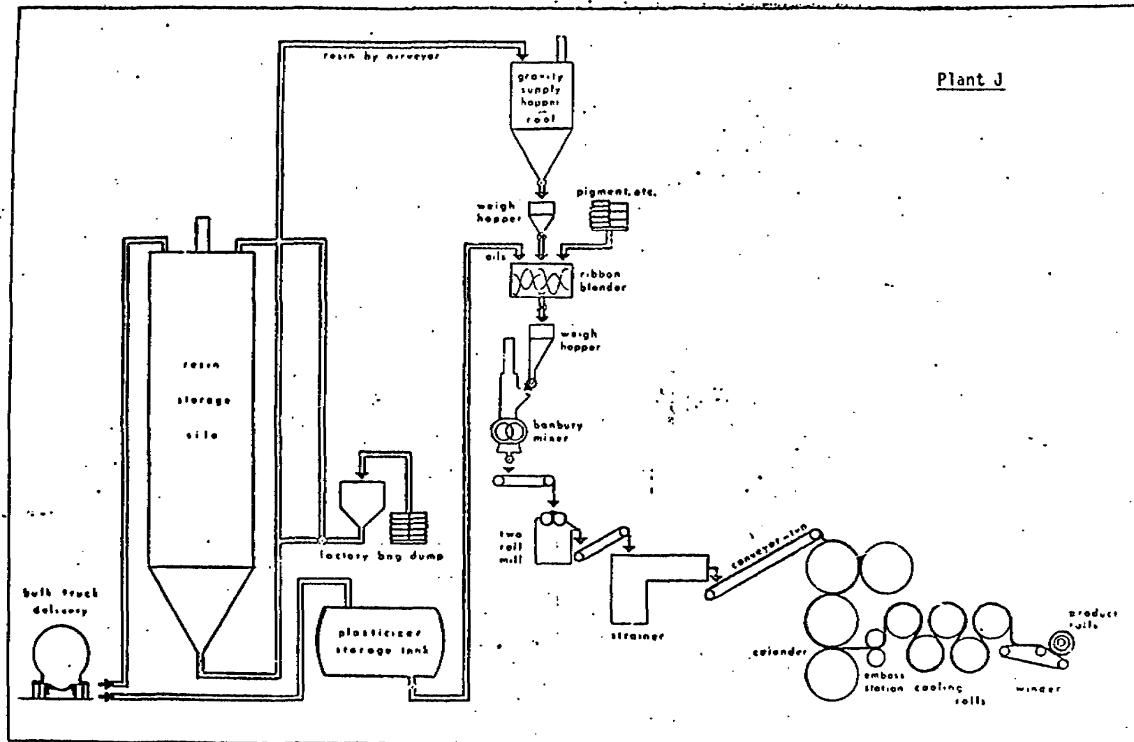
Figure 14. Flow Schematic; Calendered Film Production, Plant J
