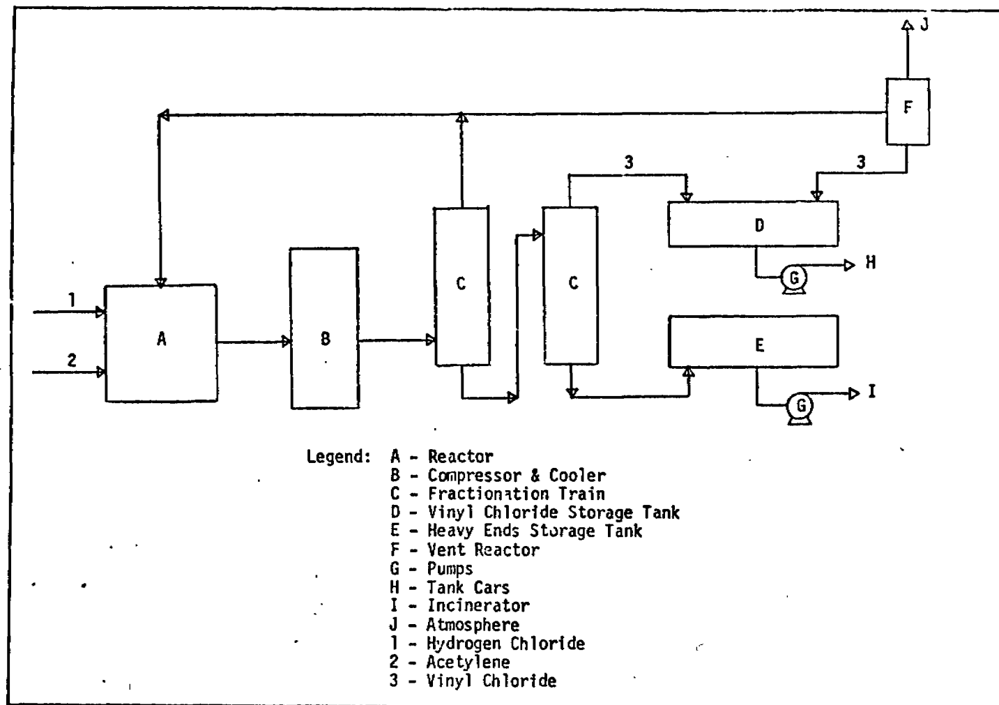
Figure 1. Acetylene-Hydrogen Chloride Process
