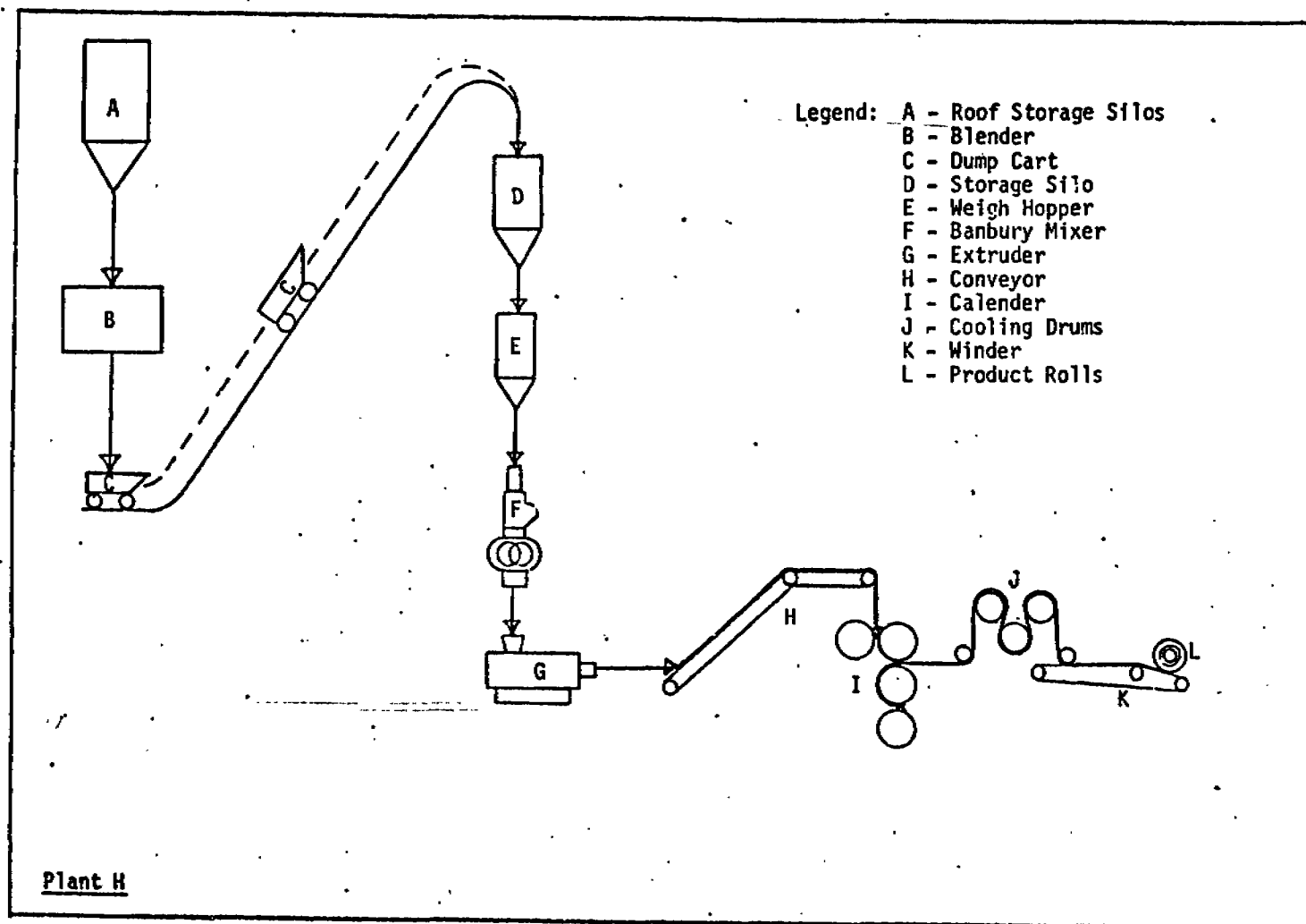
Figure 11. Flow Schematic, Plant H
