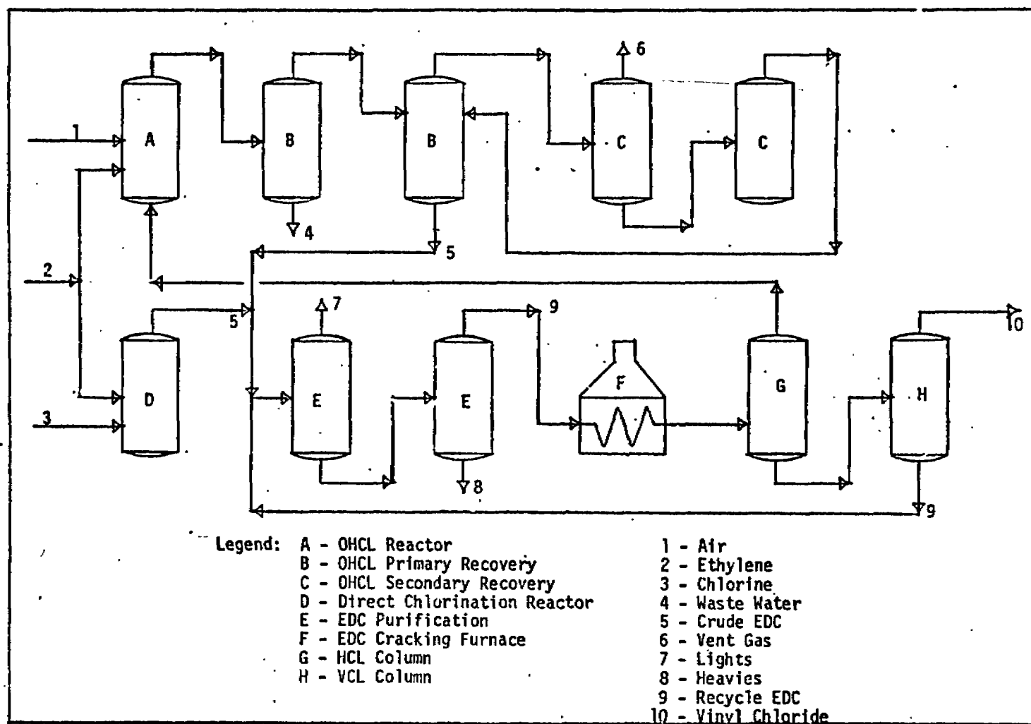
Figure 3. Oxyhydrochlorination Process
