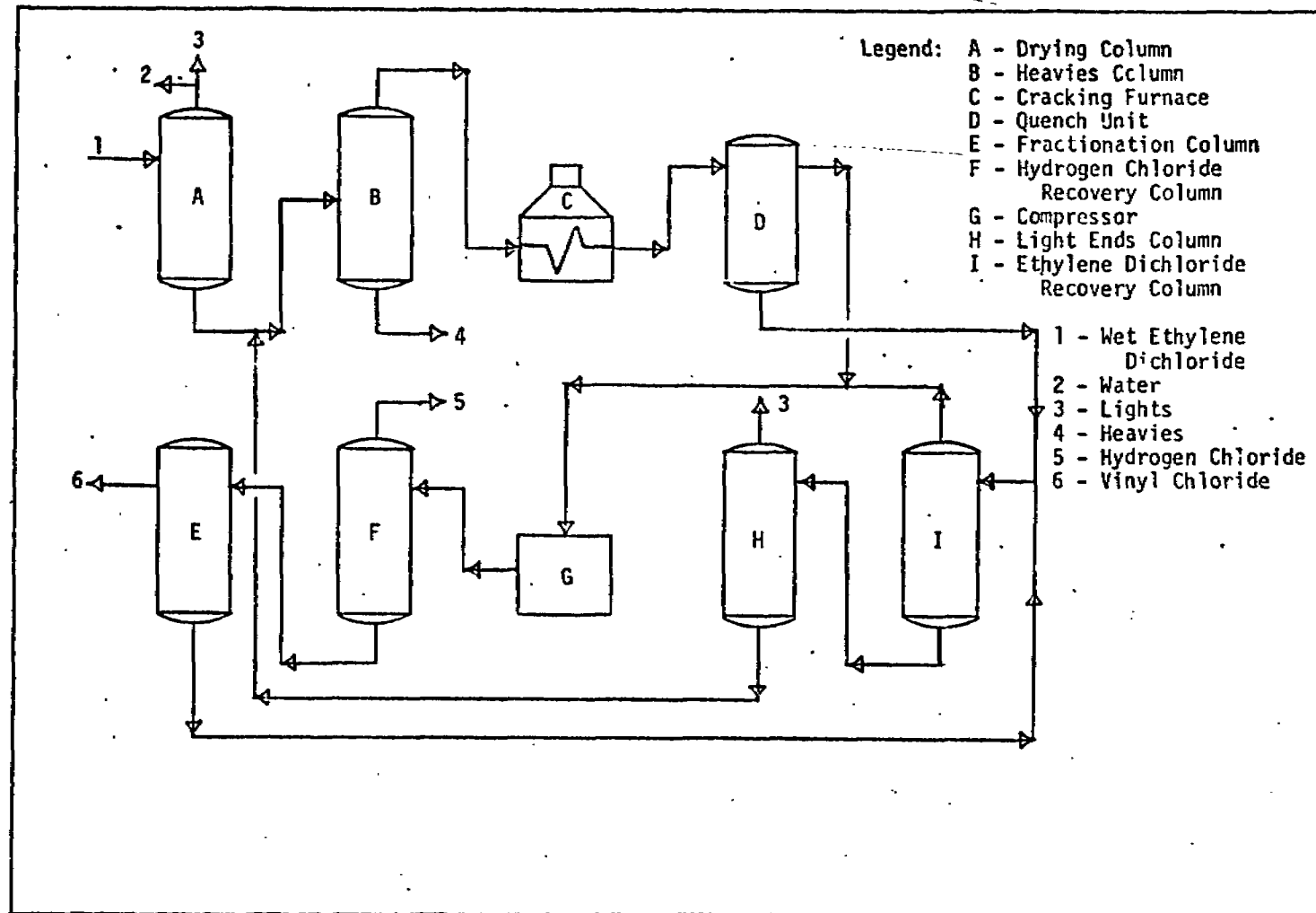
Figure 2. Ethylene Dichloride Pyrolysis Process
