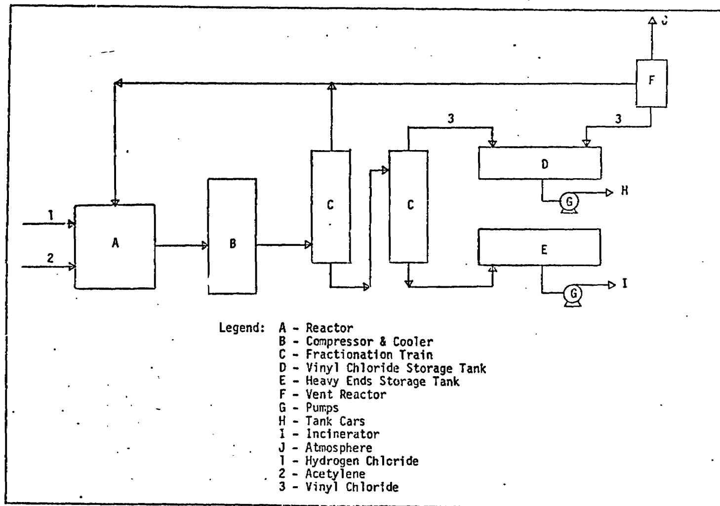
Figure 4. Flow Schematic, Plant A
