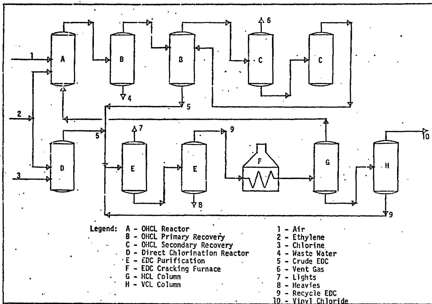
Figure 6. Flow Schematic, Plant C
