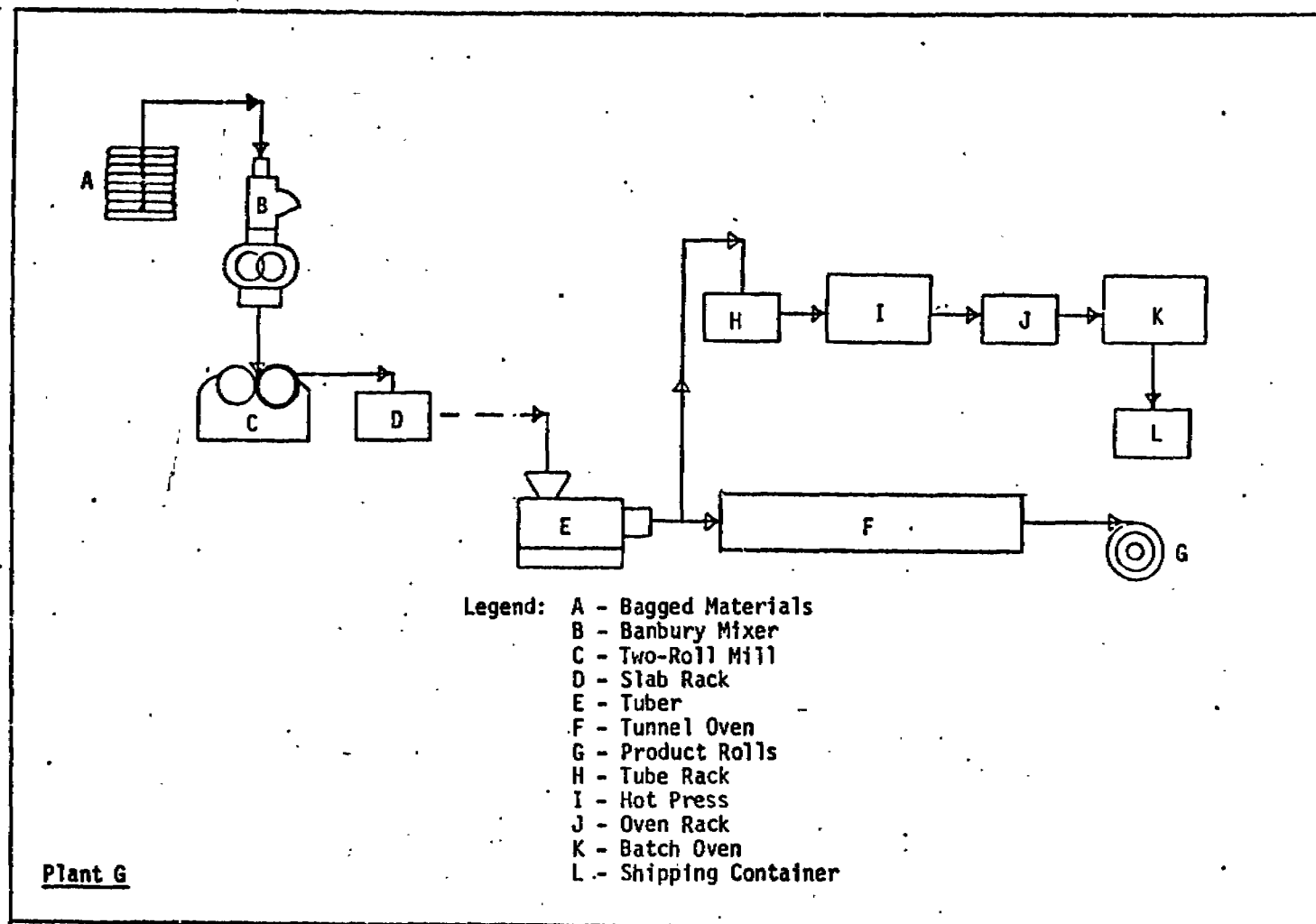
Figure 10. Flow Schematic, Plant G
