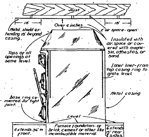
FIG. 5. DETAILS OF FURNACE BONNET, CASING, AND FOUNDATION (FROM GRAVITY CODE AND MANUAL)
