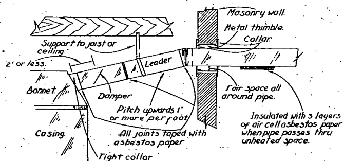
FIG. 6. DETAILS OF BONNET AND LEADER OF GRAVITY WARM-AIR FURNACE (FROM GRAVITY CODE AND MANUAL)
