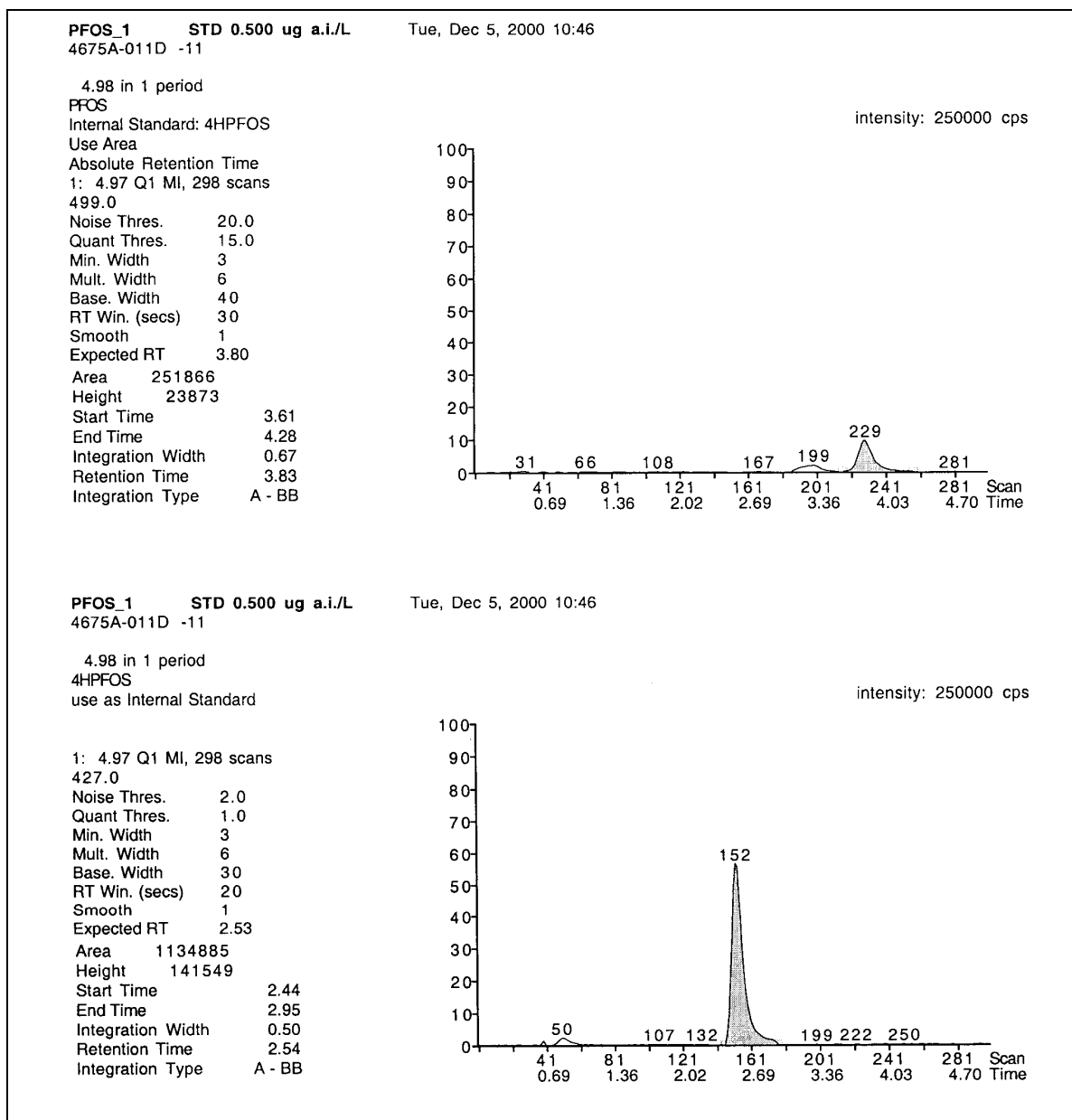
Figure 5. A representative ion chromatogram of a low-level (0.500 \mu\text{g} a.i./L) Perfluorooctanesulfonate, Potassium Salt (PFOS) standard for freshwater analyses. (monitored masses = 499 amu (PFOS - top) and 427 amu (4HPFOS internal standard - bottom)).
