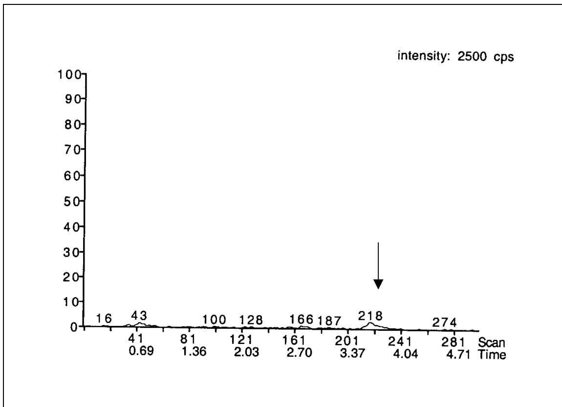
Figure 13. A representative ion chromatogram of a nonedible fish tissue matrix blank sample (454A-134-N-MAB-1, overall dilution factor = 100 L/Kg). The arrow indicates the retention time of Perfluorooctanesulfonate, Potassium Salt (PFOS). (monitored mass = 499 amu \rightarrow 99.1 amu).
