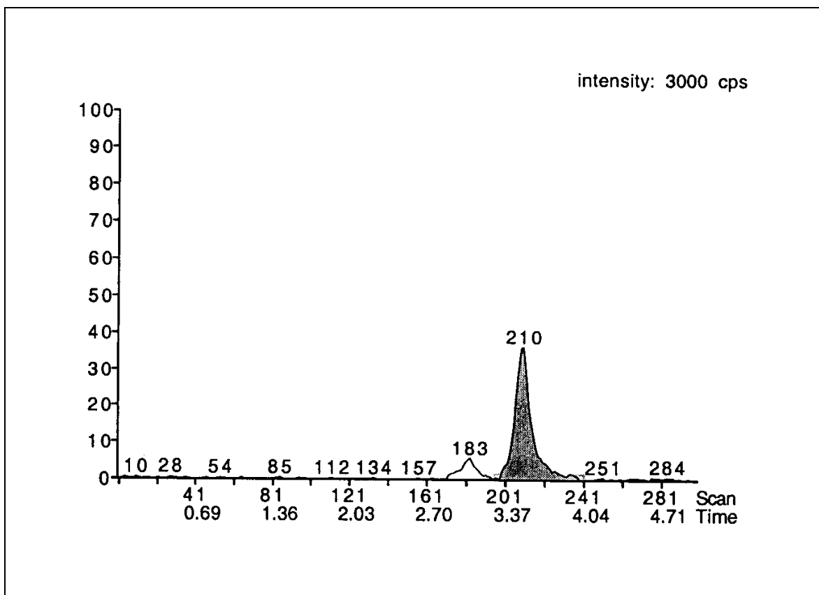
Figure 15. A representative ion chromatogram of a nonedible fish tissue matrix fortification sample (454A-134-N-MAS-8, 100 mg a.i./Kg nominal concentration, overall dilution factor = 50000 L/Kg). (monitored mass = 499 amu → 99.1 amu).
