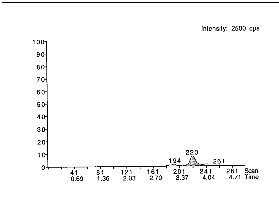
Figure 8. A representative ion chromatogram of a low-level (0.500 µg a.i./L) Perfluorooctanesulfonate, Potassium Salt (PFOS) standard for fish tissue analyses. From low-range (0.500 to 5.00 µg a.i./L) calibration set. (monitored mass = 499 amu → 99.1 amu).
