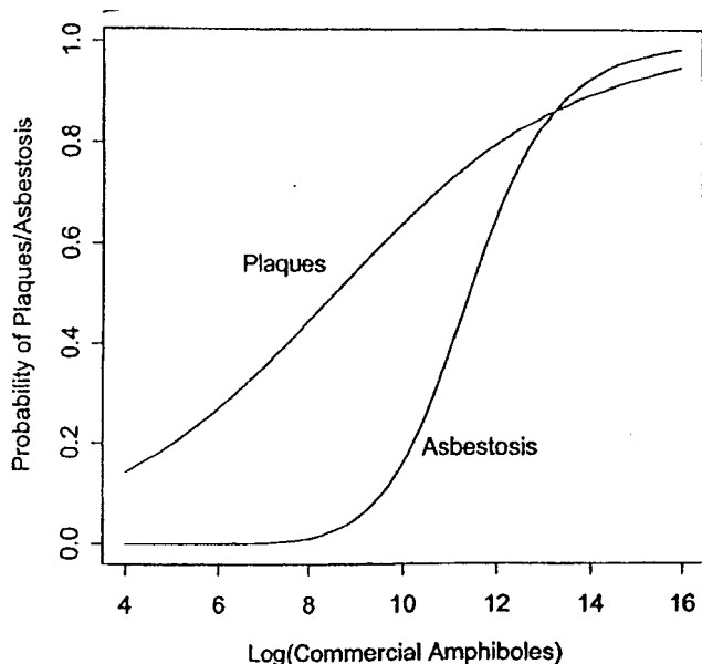
FIG. 4 Plots of the probability of either observing pleural plaques or asbestosis on the vertical scale versus log (commercial amphiboles) found per gram of tissue on the horizontal scale. The lines provide a graphical picture of the results of two logistic regression equations (see equations 1 and 2), one for the probability of observing plaques (left curve, as noted) and one for the probability of observing asbestosis (right curve, as noted).
