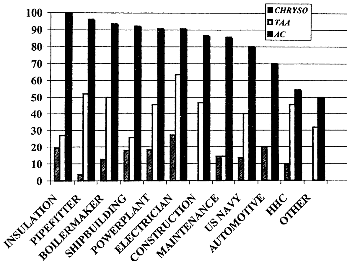
FIG. 3 Histogram showing the percentage of cases in each category with elevated lung fiber burdens for commercial amphiboles (AC), noncommercial amphiboles (TAA), and chrysotile. Categories represented are those for which at least 10 cases with lung analyses in the given category were available. HHC, household contact.
