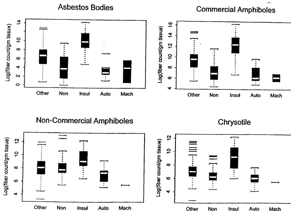
FIG. 2 Boxplots of fiber burden for asbestos bodies (upper left), commercial amphiboles (upper right), noncommercial amphiboles (lower left), and chrysotile fibers. The vertical axis provides the fiber burdens in log (number per gram), and each plot provides the details for 5 industrial or occupational groups: nonindustrial exposure (Non), insulation industry (Insul), automobile industry (Auto), machinists (Mach), and all remaining groups (Other). The results inside the solid dark box provide the range from the 25th to 75th percentiles, and the white bars indicate the median value. The more distant brackets and lines above and below the solid boxes provide the full range and most peripheral values.
