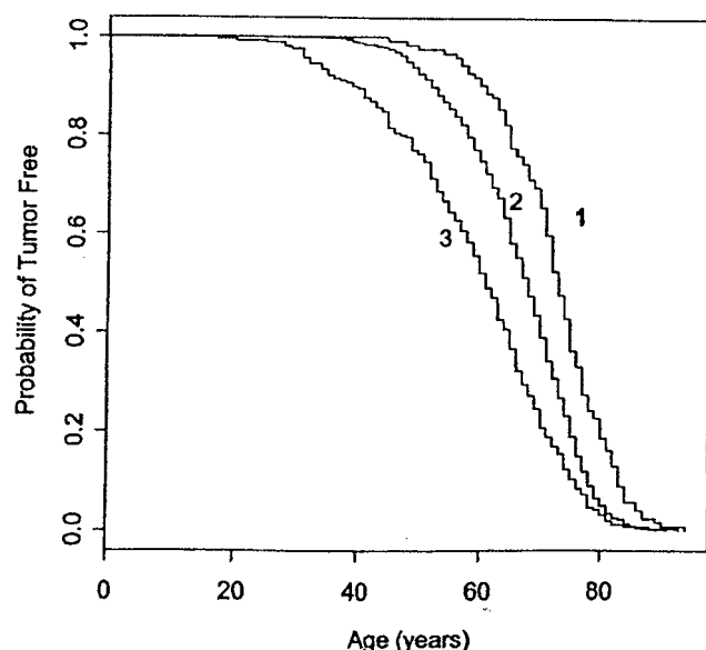
FIG. 1 Kaplan-Meier plots of the probability of being tumor free versus age in years. Here age at diagnosis was treated as a failure time. Curve 1 provides the plot for pipefitters and railroad workers; curve 3 provides the plot for those in the insulation industry and those with nonindustrial exposure; and curve 2 provides the plot for the remaining groups of industrial/occupational exposures.
