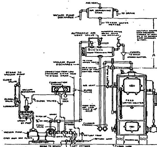
FIG. 43. METHOD OF CONNECTING VACUUM PUMP, FEED WATER HEATER AND SINGLE CONTROL HYDRO-PNEUMATIC TANK OR AIR SEPARATING TANK
