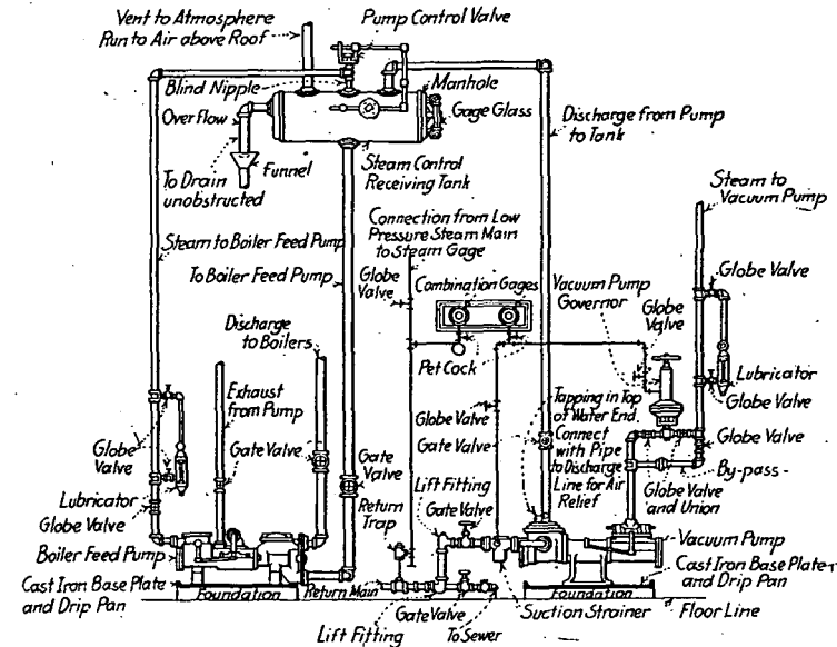
FIG. 45. METHOD OF CONNECTING VACUUM PUMP, BOILER-FEED PUMP AND STEAM-CONTROL RECEIVING TANK
