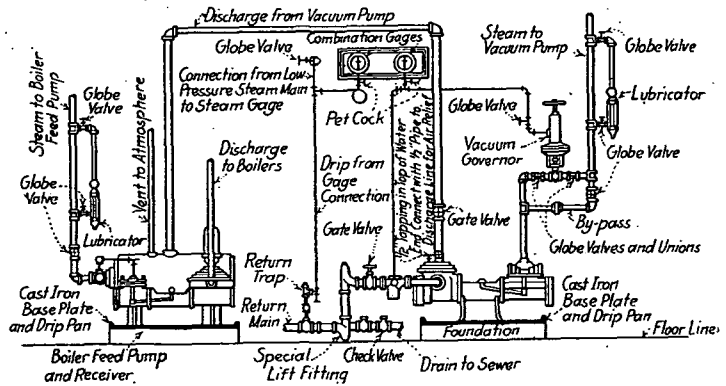
FIG. 44. METHOD OF CONNECTING VACUUM PUMP AND AUTOMATIC BOILER-FEED PUMP AND RECEIVER
