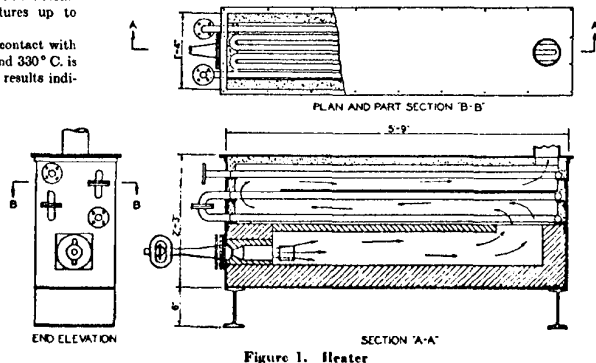
Figure 1. Heater
