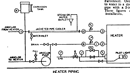
Figure 2. Cooler, Pump, and Expansion Tank
