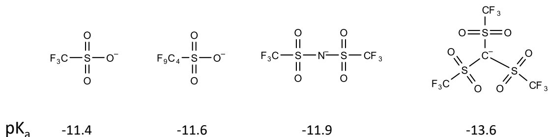
Figure 10: Modern C1 anions suitable for use in advanced resists: bis-trifluoromethylsulfonamide and tris-(trifluoromethylsulfonyl) methide anions, respectively, and the acid dissociation constant ( \text{pK}_a ) values of the conjugated acids (on the 1,2-dichloroethane scale) compared to trifluoromethane sulfonate and PFBS (left) (Paenurk, et al. 2017). The two C1 acids meet or exceed the strength of PFBS, while showing similar diffusivity and a lack of side reactions in CARs.
