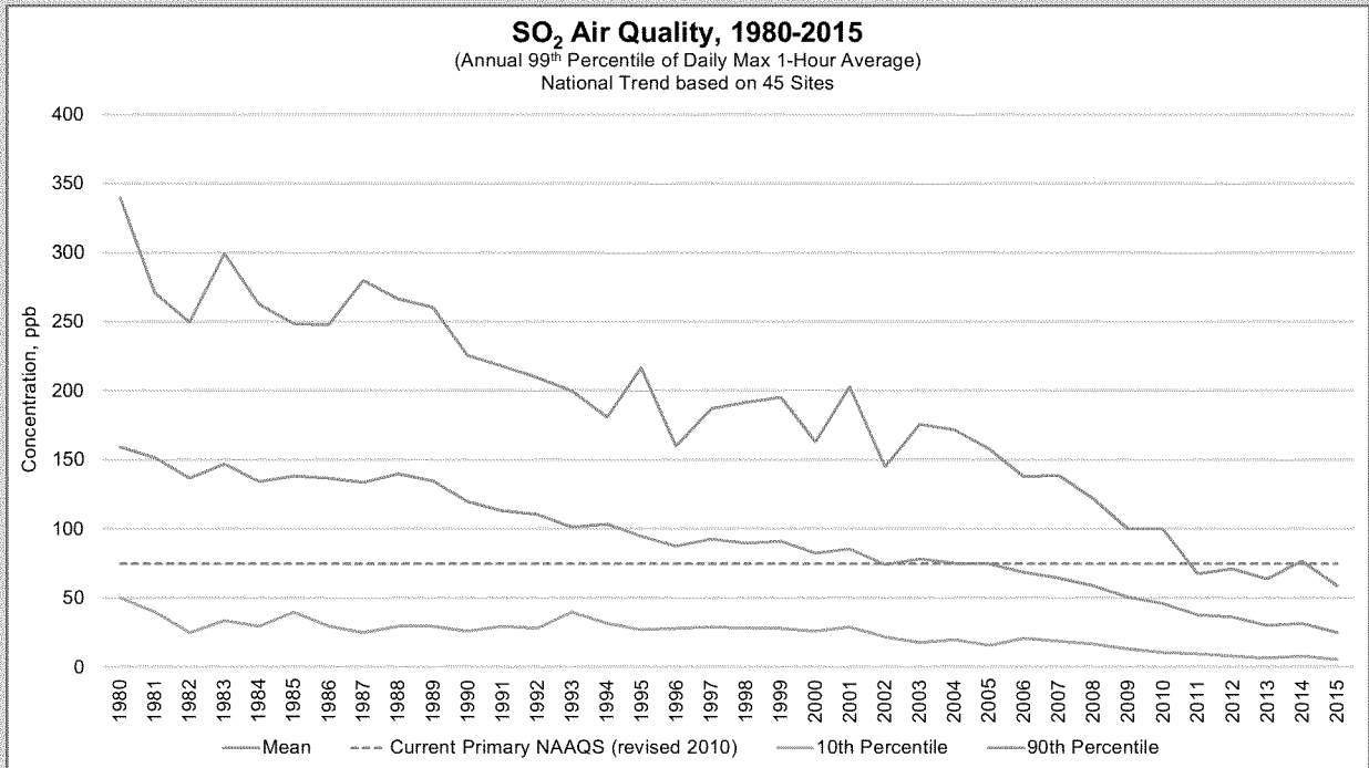
Source: U.S. EPA, Sulfur Dioxide Trends .
