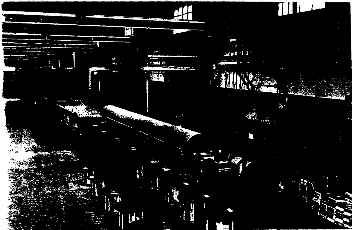
One of two electroplating lines at Camden Wire used for coating copper wire with a tin-lead alloy for easier manufacture of printed circuit boards.
