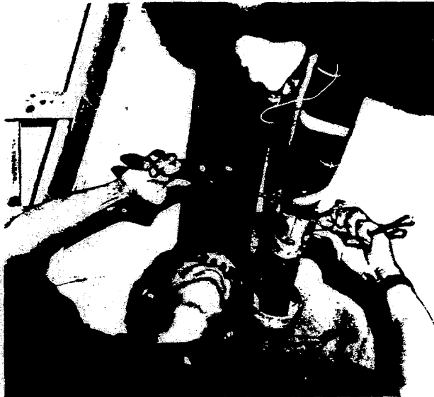
Even unskilled workers can quickly learn to make splices in the lead sheathed cable with a modification of the electrical wipe system.
