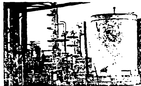
Trickling filter tower containing Surfpac plastic biological oxidation media (in Dow's Bay City, Michigan, petrochemical plant) performs same function as rock trickling filter but requires less land area.
