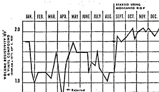
Test showing variation of volume resistivity with time. Note change when Monsanto became supplier.
