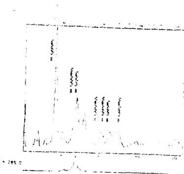
Figure 2. Reconstructed chromatograms of urine extracts from rats fed a diet of Aroclor 1016. 3% OV-1 column programmed from 150° to 210° at 2° per minute.
