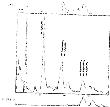
Figure 1. Reconstructed chromatograms of urine extracts from rats fed a diet of Aroclor 1242. 3% OV-1 column programmed from 150° to 210° at 2° per minute.
