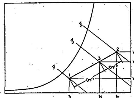
FIG. 11. SOLUTION OF EXAMPLE 5 ON A.S.H.A.E. PSYCHROMETRIC CHART
