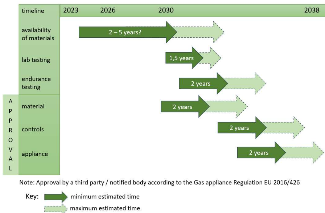
Figure 1: estimated time frame needed for the replacement of fluoropolymer containing components in afecors' controls and the release of certified controls with alternative materials (best case scenario)
