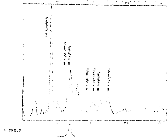
Figure 2. Reconstructed chromatograms of urine extracts from rats fed a diet of Aroclor 1016. 3% OV-1 column programmed from 150° to 210° at 2° per minute.
